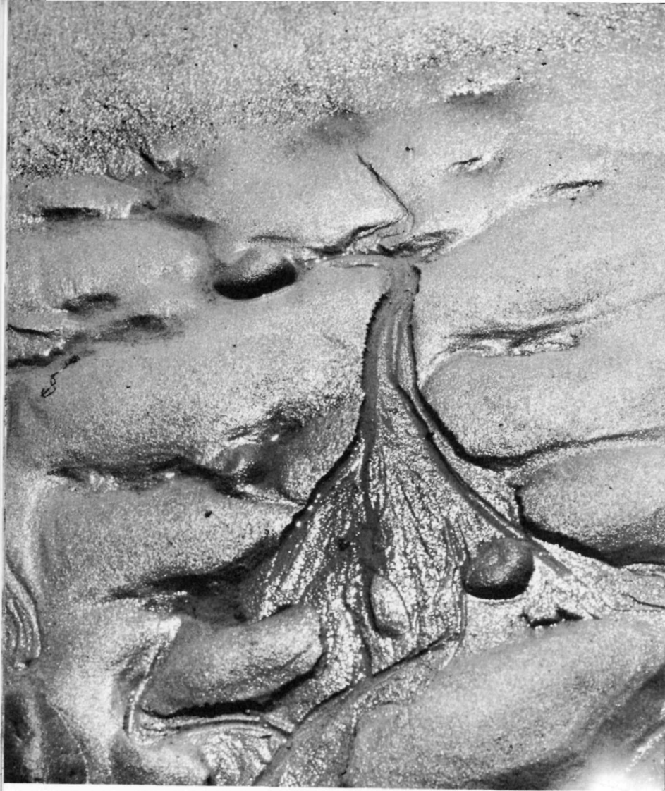
Figure 6. When the tide goes out, water left in the sands of the sloping beach gradually runs out and sometimes collects to form a small stream like this one.
