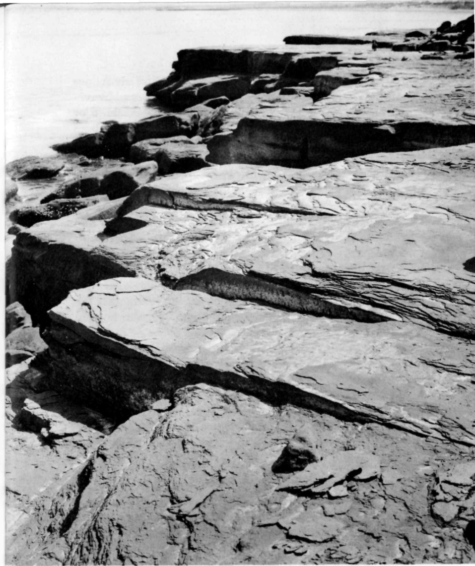
Figure 1. Sandy red siltstone and sandstone form the coastline west of North Rustico. The thin layering parallels the ancient surface on which these sedimentary materials were laid down some 250 million years ago. The rocks are broken by vertical fractures or joints which can be seen trending diagonally across the picture.
