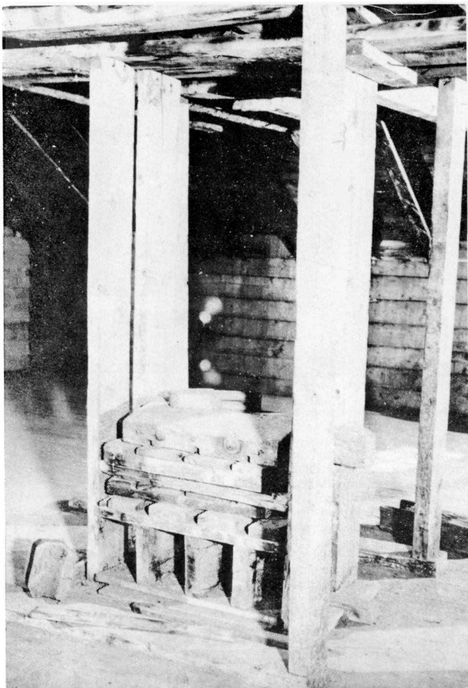
Fur press used for pressing the pelts to bale for shipment By permission of the Hudson's Bay Company
