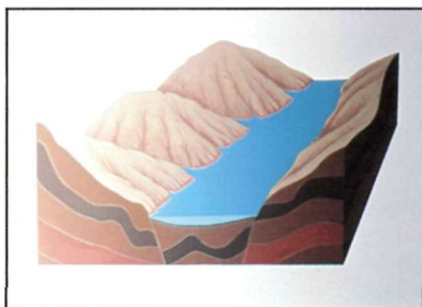
Fig. 2: Shallow sea
