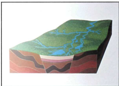
Fig. 4: Coal-age swamps
