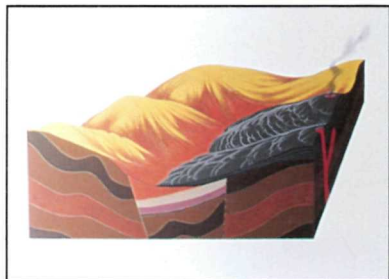
Fig. 5: Volcanoes erupt
