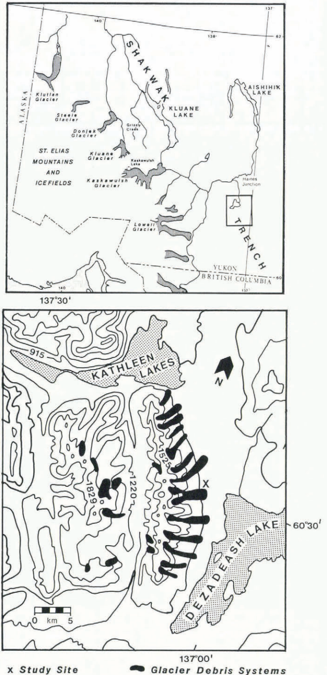
Fig. 1. Location of the glacier ice-cored rock glaciers and the study site in the Dalton Range.
