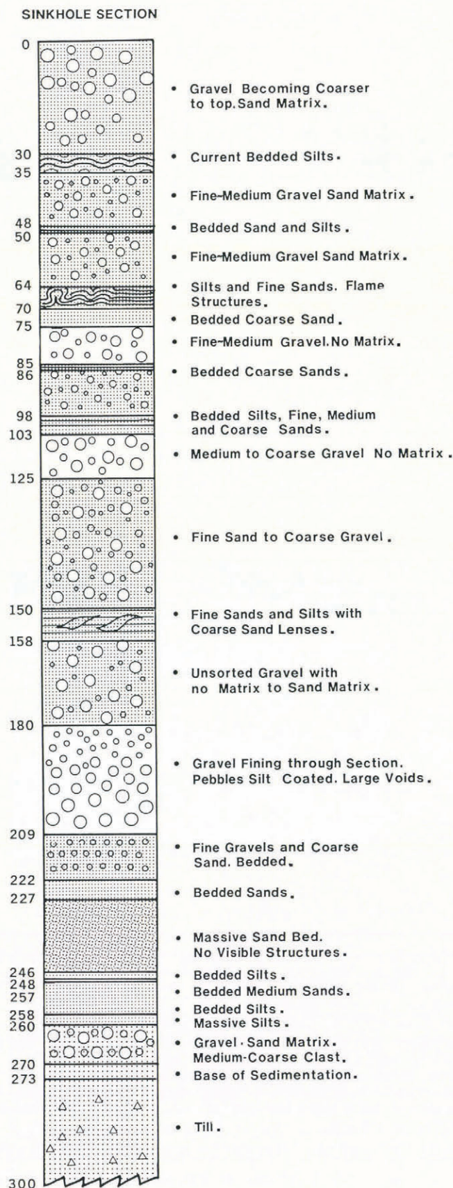
Fig. 6. The stratigraphy of the deposits in the large sink-hole.
