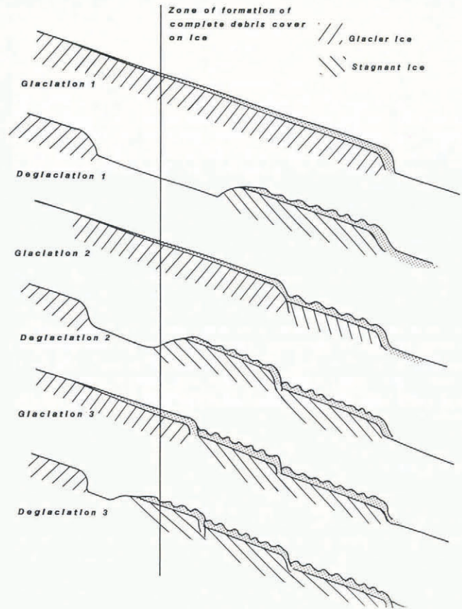
Fig. 7. Schematic of the formation of glacier ice-cored rock glaciers by periods of glacier advance.
