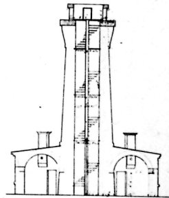
Section of Tower & Buildings on the Line A-B
