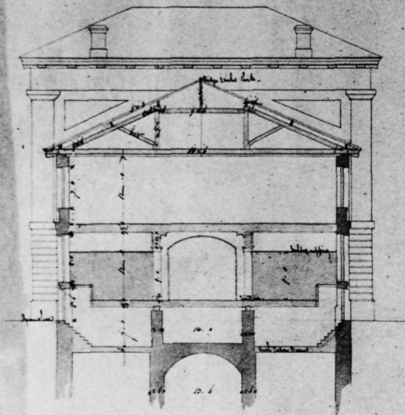
TRANSVERSE SECTION
